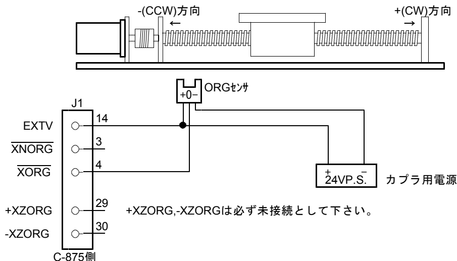
(1) ORG-0,ORG-1,ORG-2,ORG-3型式時(X軸)
